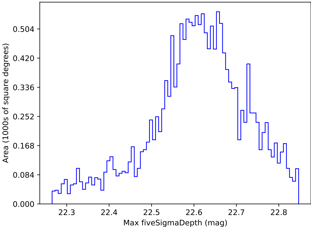
too_ignore_10_1v3.4_10yrs WFD y band: Max fiveSigmaDepth
