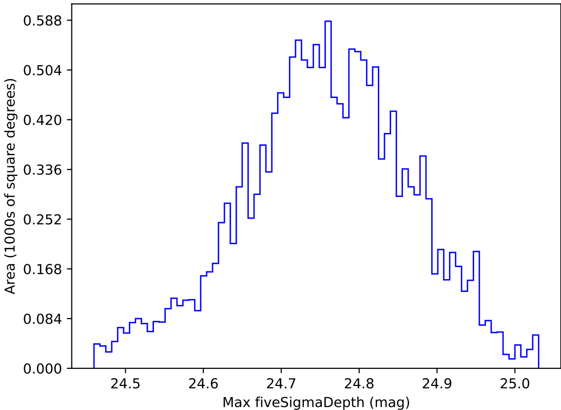
too_ignore_10_1v3.4_10yrs WFD r band: Max fiveSigmaDepth
