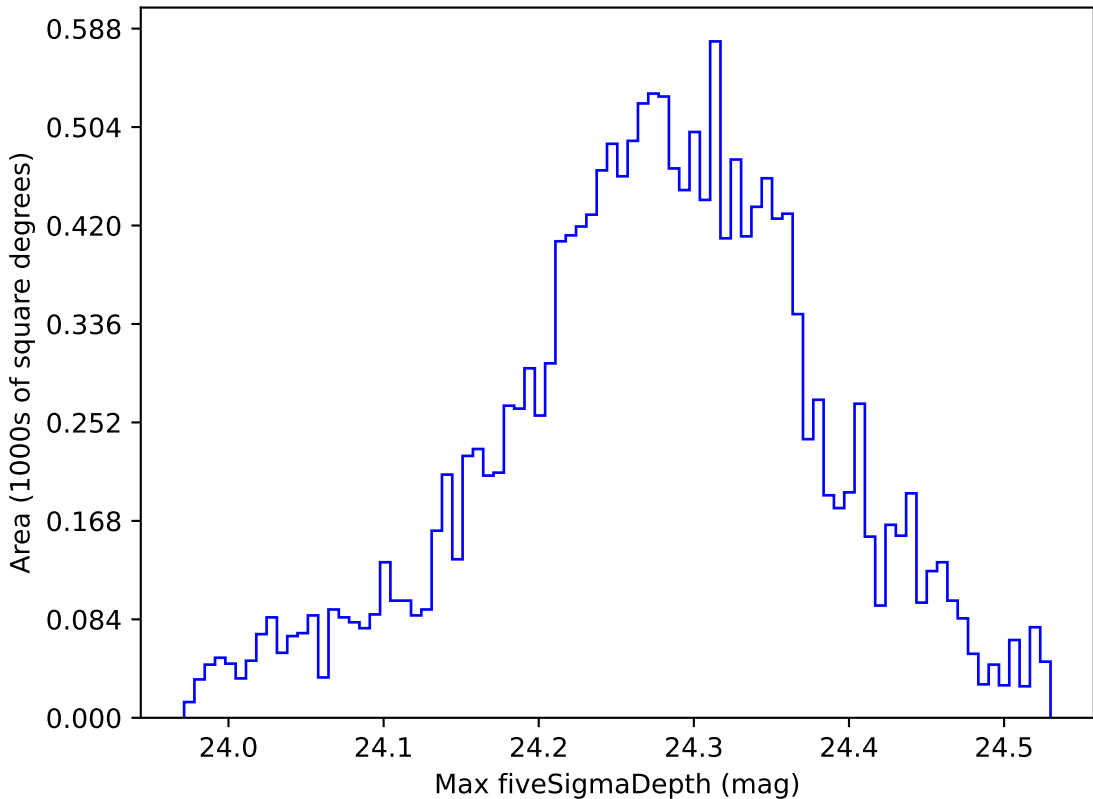
too_ignore_10_1v3.4_10yrs WFD i band: Max fiveSigmaDepth
