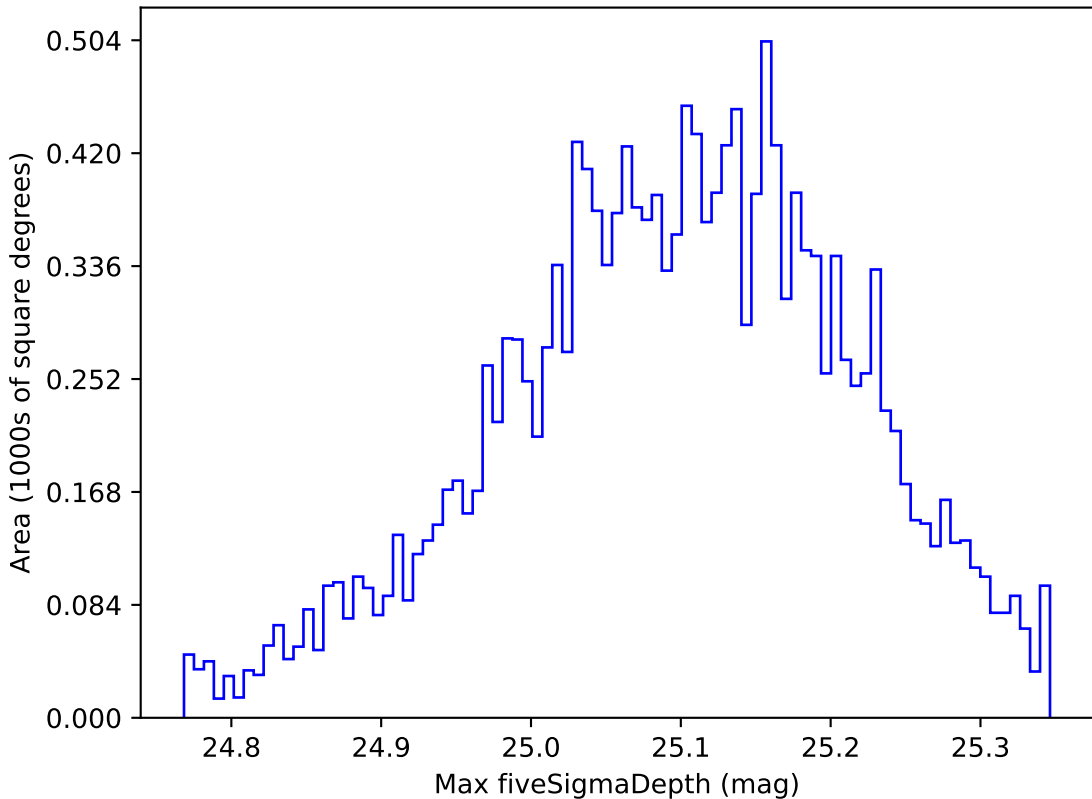
too_ignore_10_1v3.4_10yrs WFD all bands: Max fiveSigmaDepth
