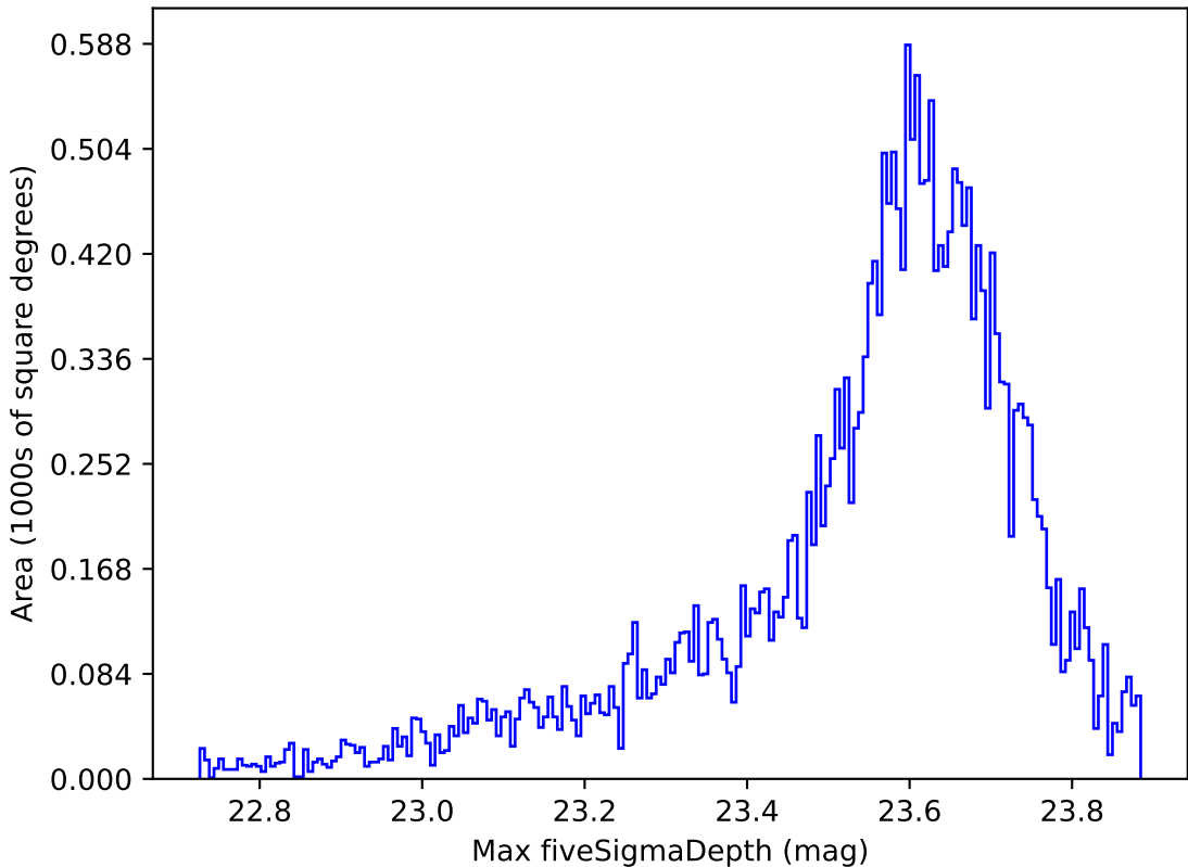
too_ignore_10_1v3.4_10yrs All sky z band: Max fiveSigmaDepth
