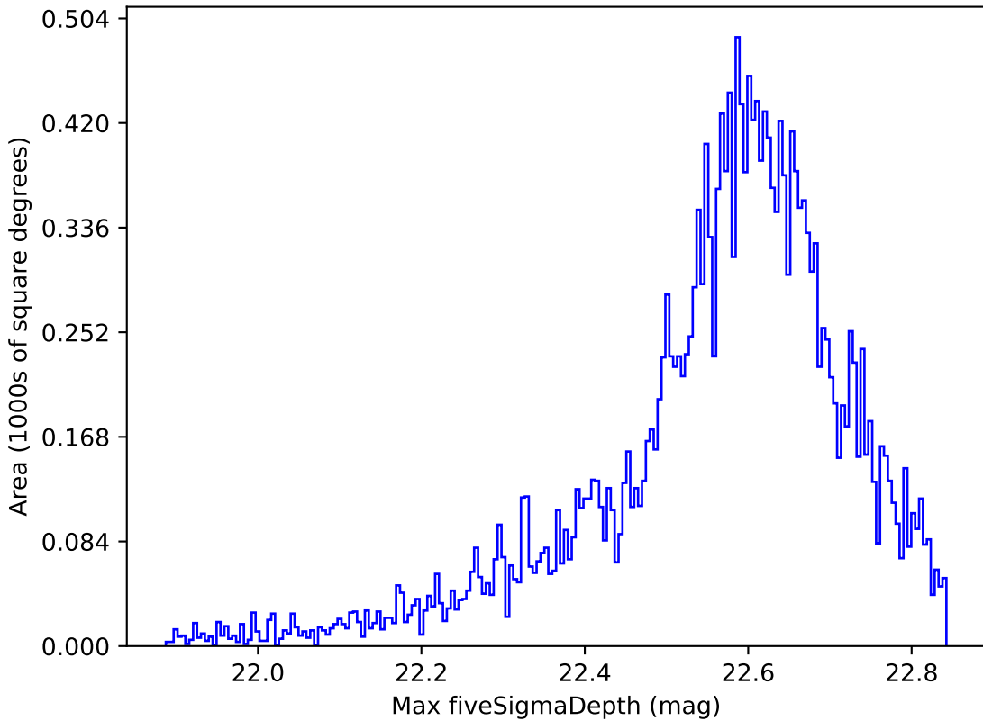
too_ignore_10_1v3.4_10yrs All sky y band: Max fiveSigmaDepth
