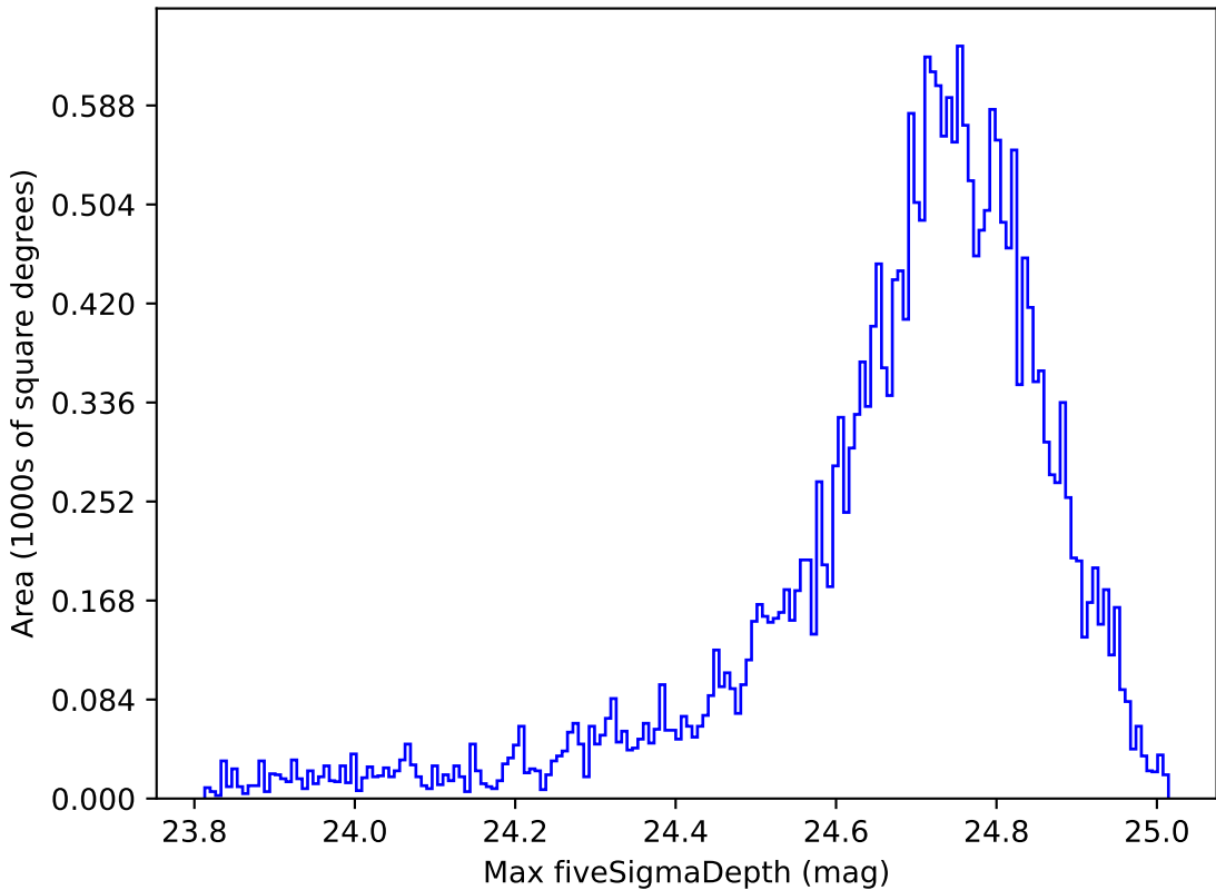
too_ignore_10_1v3.4_10yrs All sky r band: Max fiveSigmaDepth
