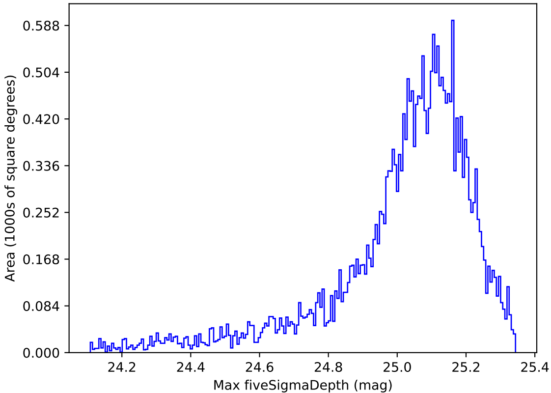
too_ignore_10_1v3.4_10yrs All sky g band: Max fiveSigmaDepth
