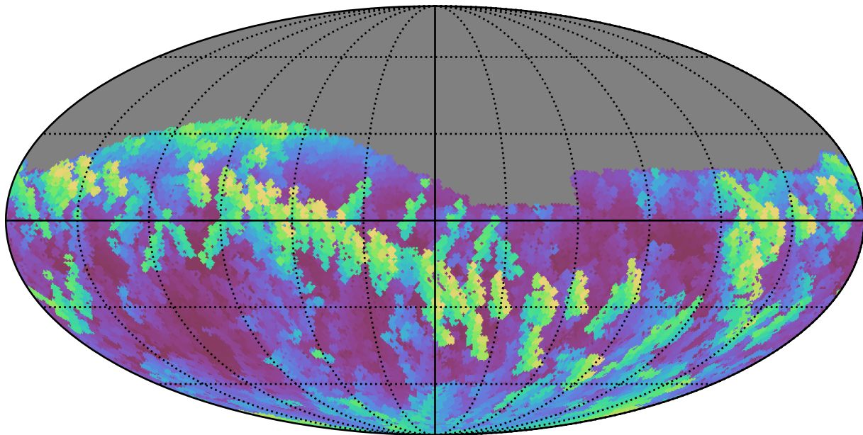
too_ignore_10_1v3.4_10yrs Yr 1 z band: Max airmass
