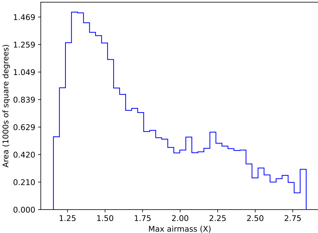
too_ignore_10_1v3.4_10yrs Yr 1 z band: Max airmass
