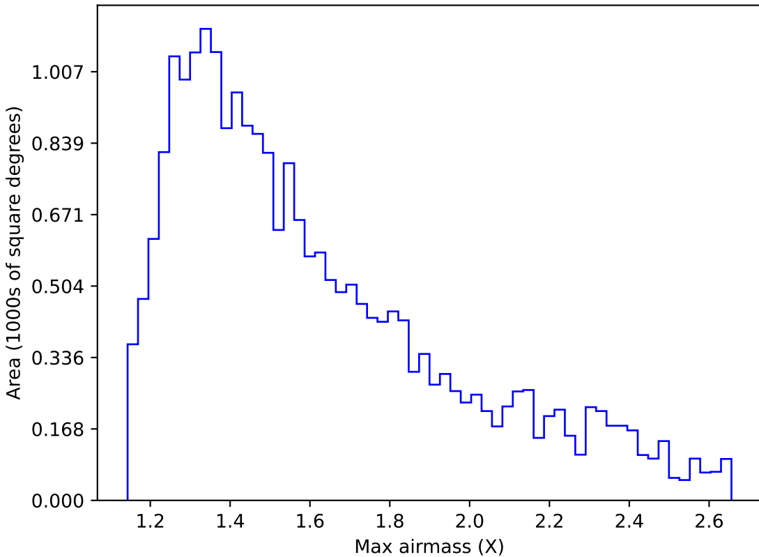
too_ignore_10_1v3.4_10yrs Yr 1 y band: Max airmass
