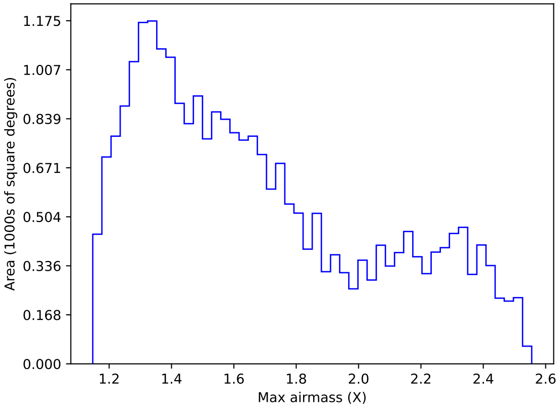
too_ignore_10_1v3.4_10yrs Yr 1 r band: Max airmass
