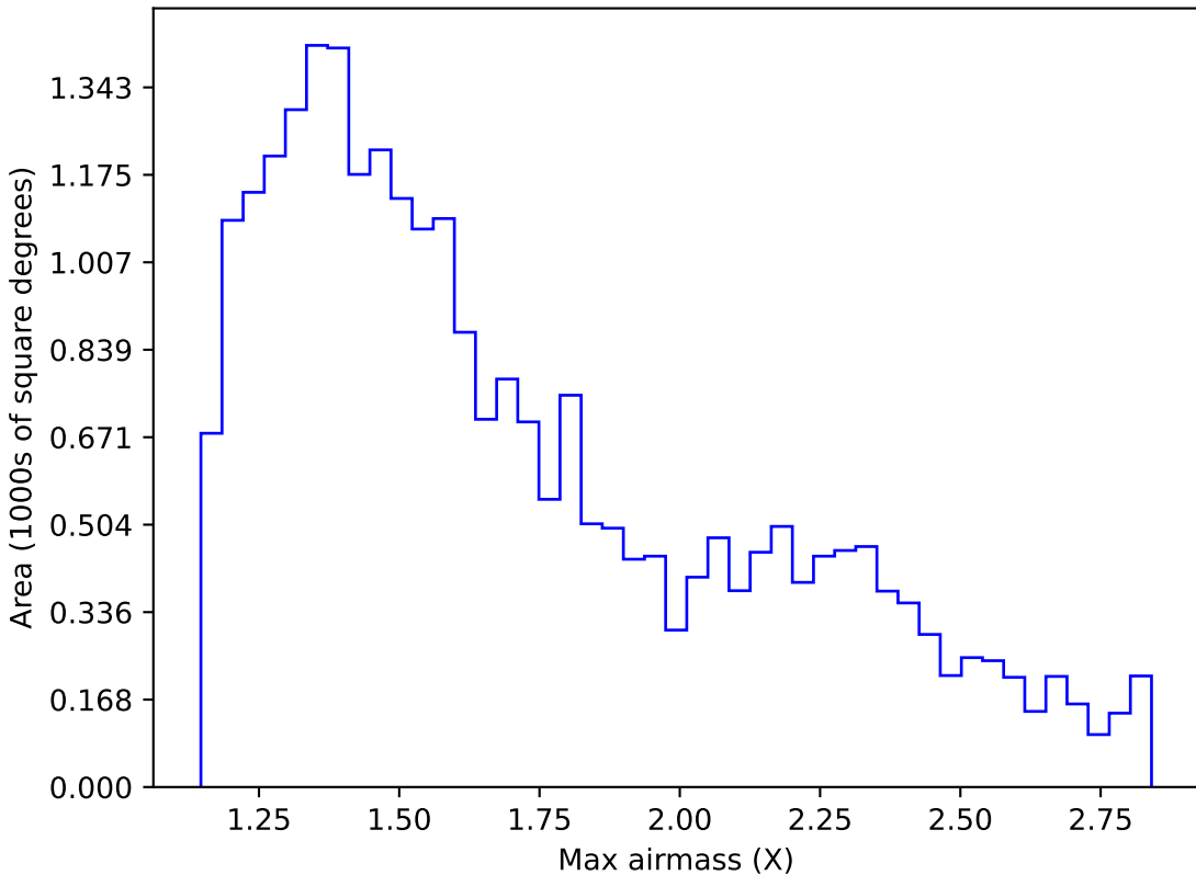
too_ignore_10_1v3.4_10yrs Yr 1 i band: Max airmass
