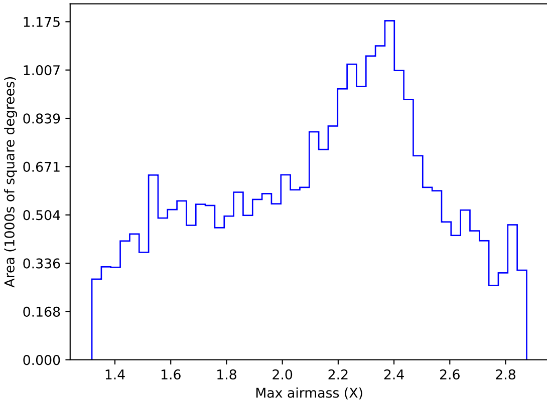
too_ignore_10_1v3.4_10yrs Yr 1 all bands: Max airmass
