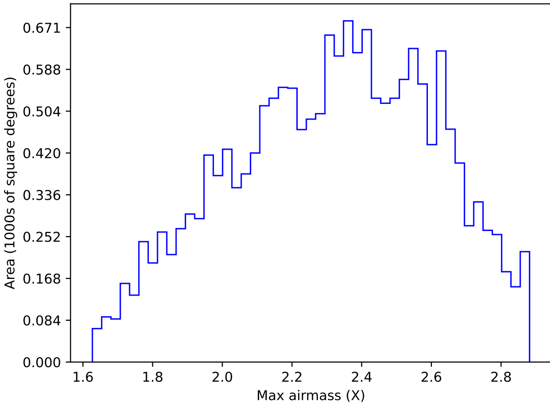
too_ignore_10_1v3.4_10yrs WFD y band: Max airmass
