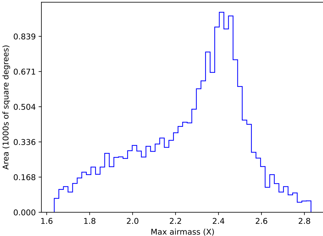
too_ignore_10_1v3.4_10yrs WFD r band: Max airmass
