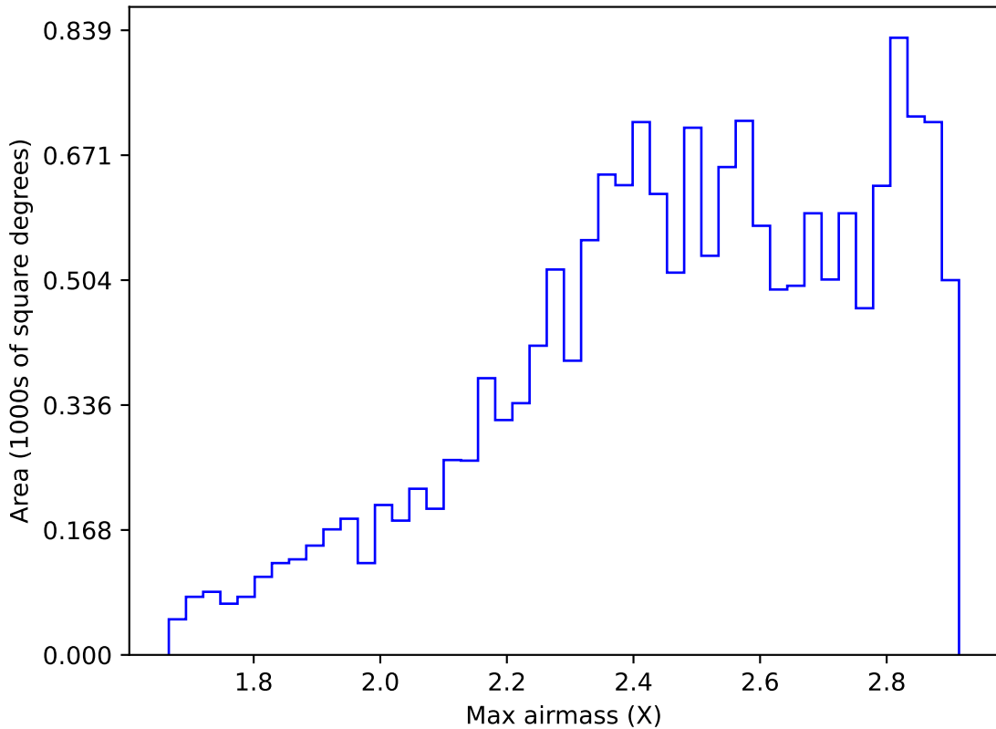
too_ignore_10_1v3.4_10yrs WFD i band: Max airmass
