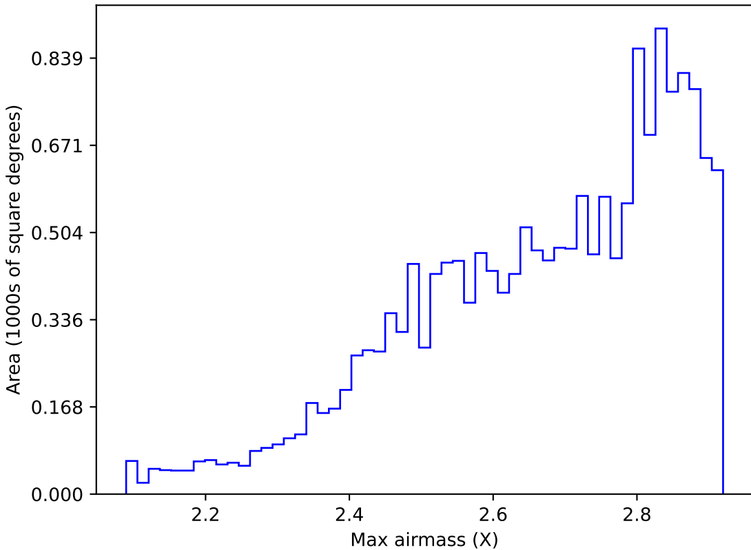
too_ignore_10_1v3.4_10yrs WFD all bands: Max airmass
