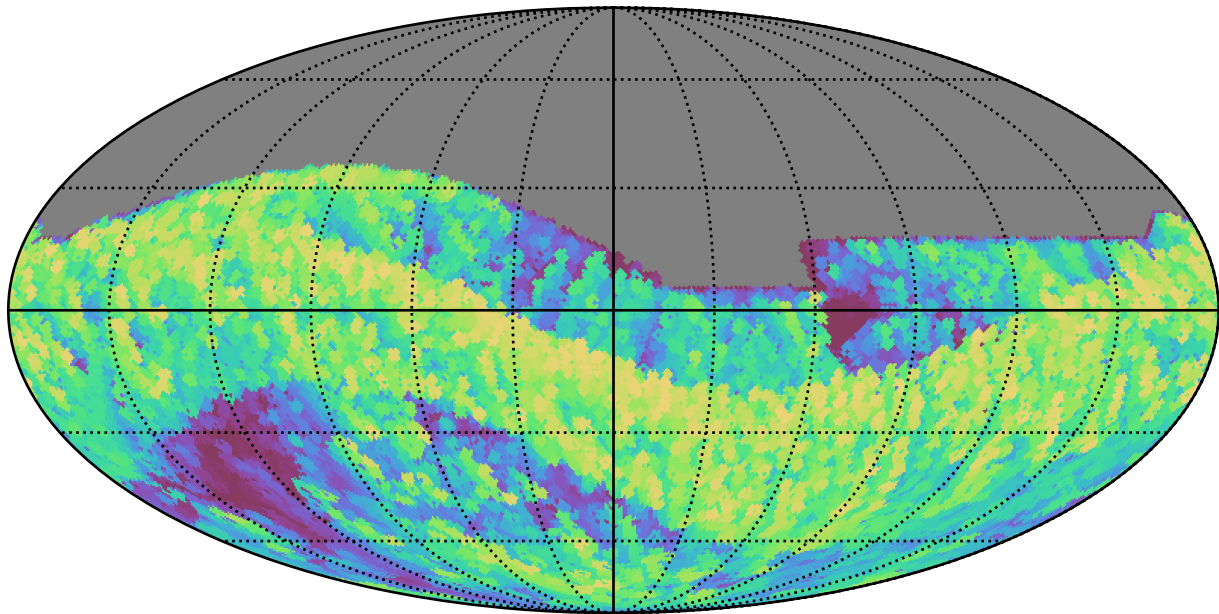
too_ignore_10_1v3.4_10yrs All sky z band: Max airmass
