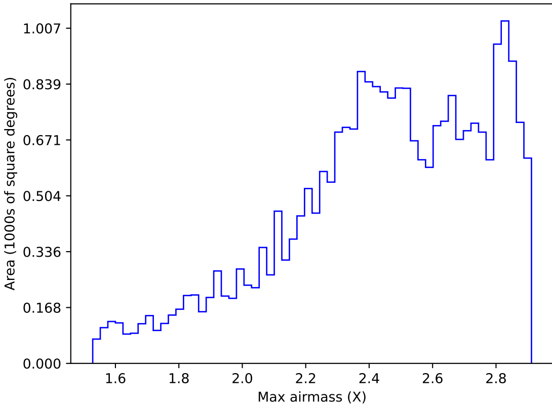
too_ignore_10_1v3.4_10yrs All sky z band: Max airmass
