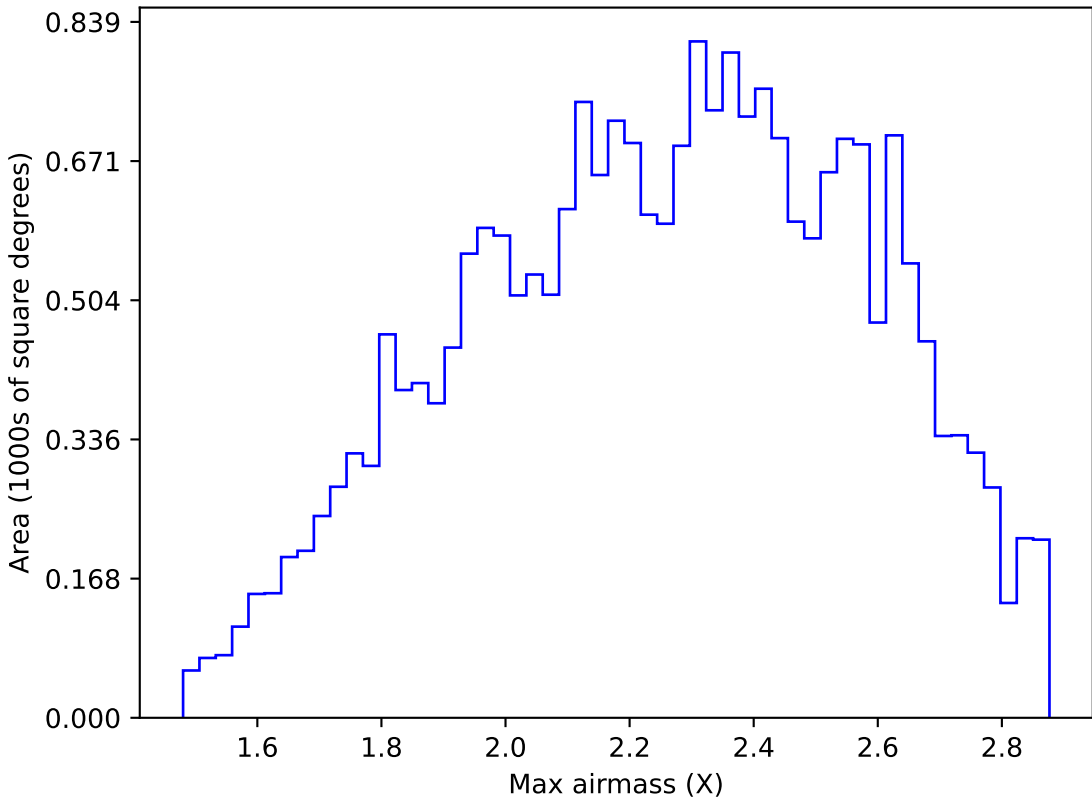
too_ignore_10_1v3.4_10yrs All sky y band: Max airmass
