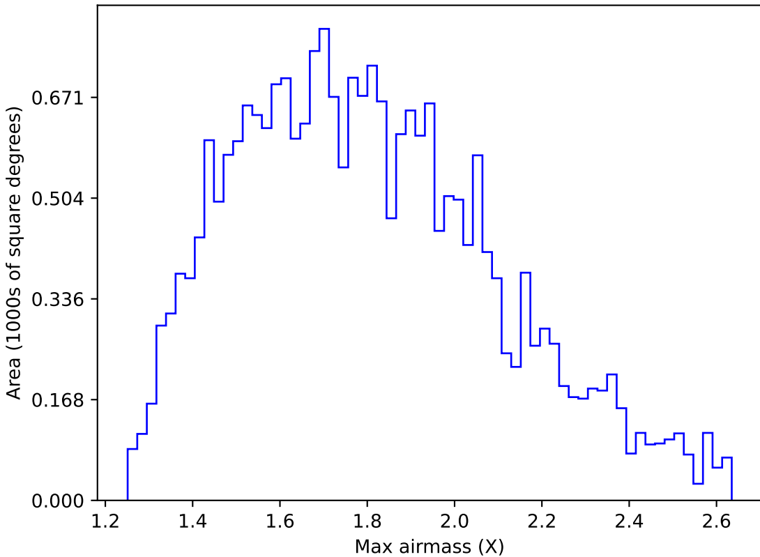
too_ignore_10_1v3.4_10yrs All sky u band: Max airmass
