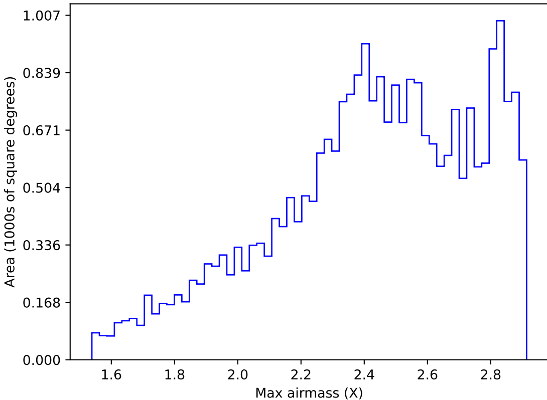
too_ignore_10_1v3.4_10yrs All sky i band: Max airmass
