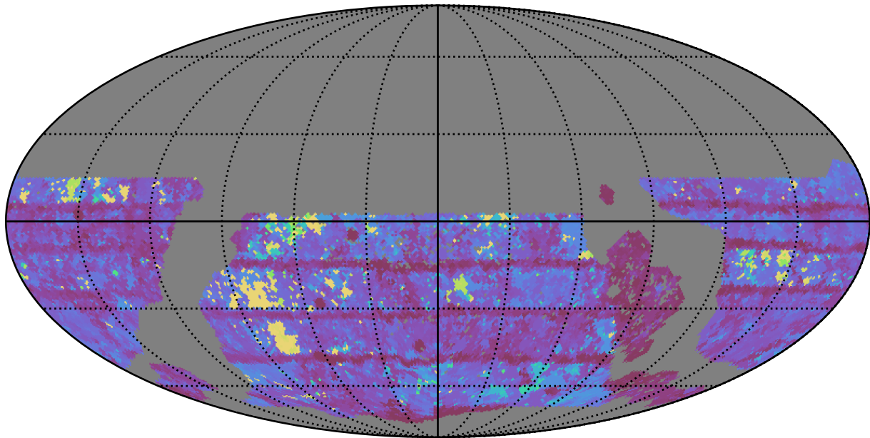
too_ignore_10_1v3.4_10yrs WFD z band: Max Inter-Night Gap
