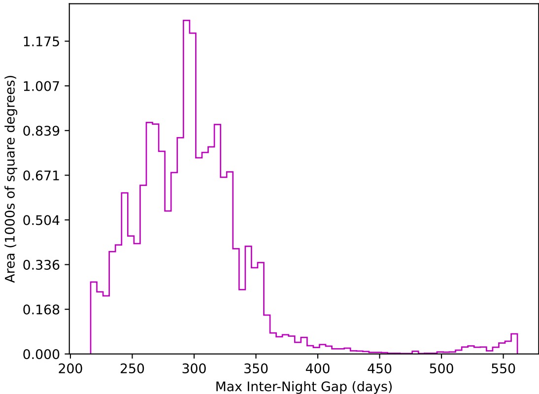
too_ignore_10_1v3.4_10yrs WFD z band: Max Inter-Night Gap
