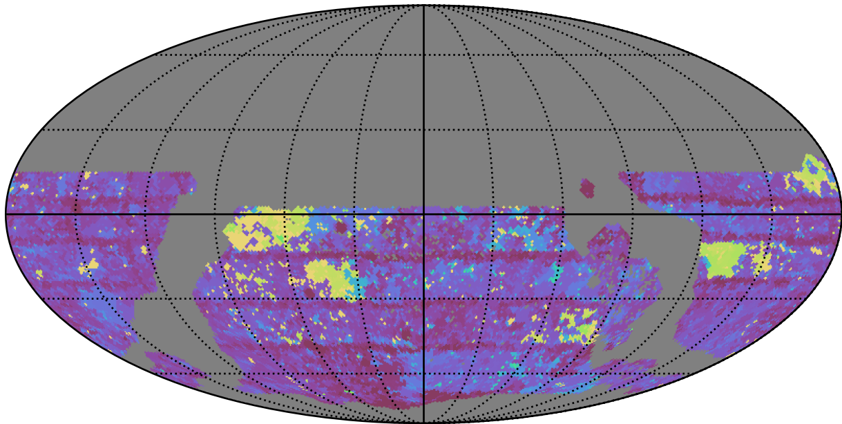
too_ignore_10_1v3.4_10yrs WFD y band: Max Inter-Night Gap
