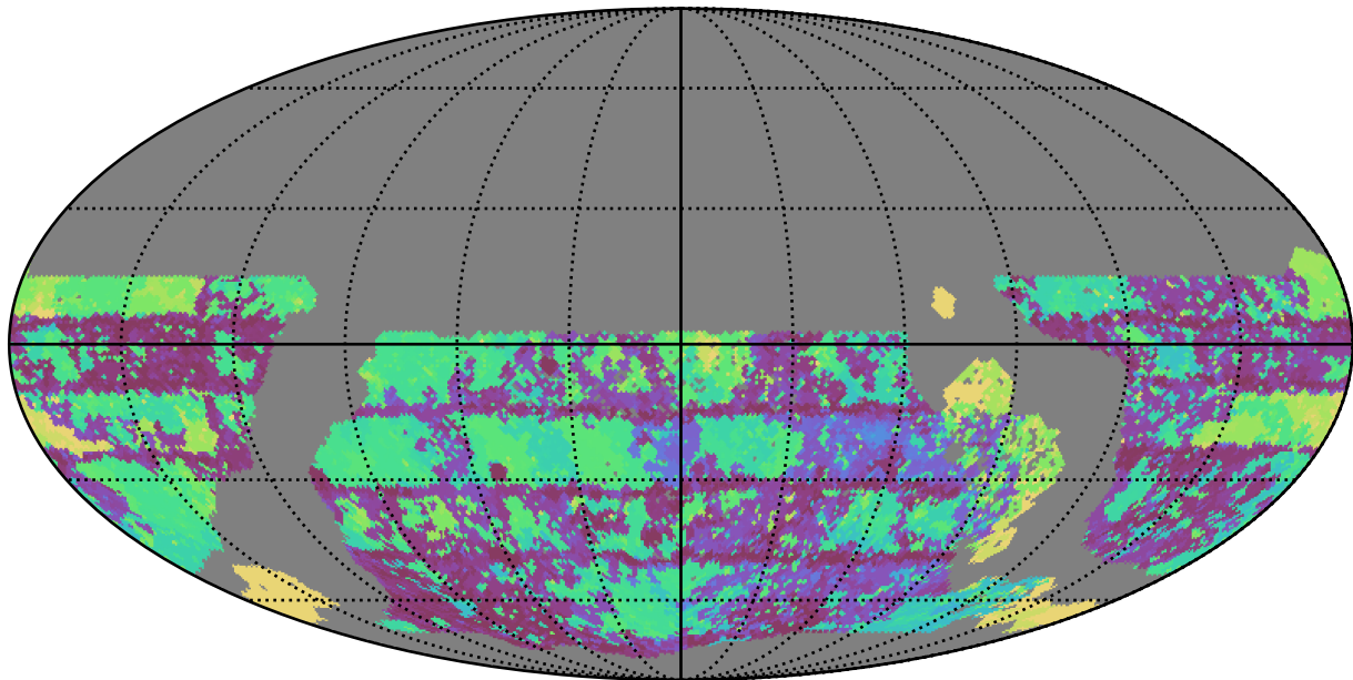
too_ignore_10_1v3.4_10yrs WFD u band: Max Inter-Night Gap
