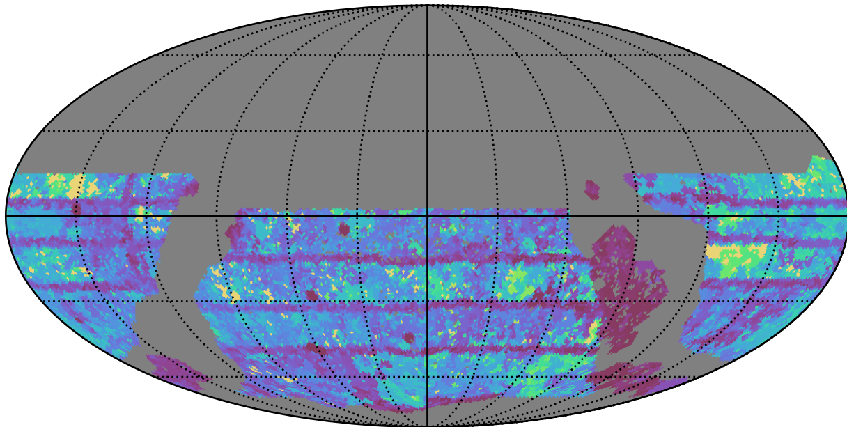
too_ignore_10_1v3.4_10yrs WFD r band: Max Inter-Night Gap
