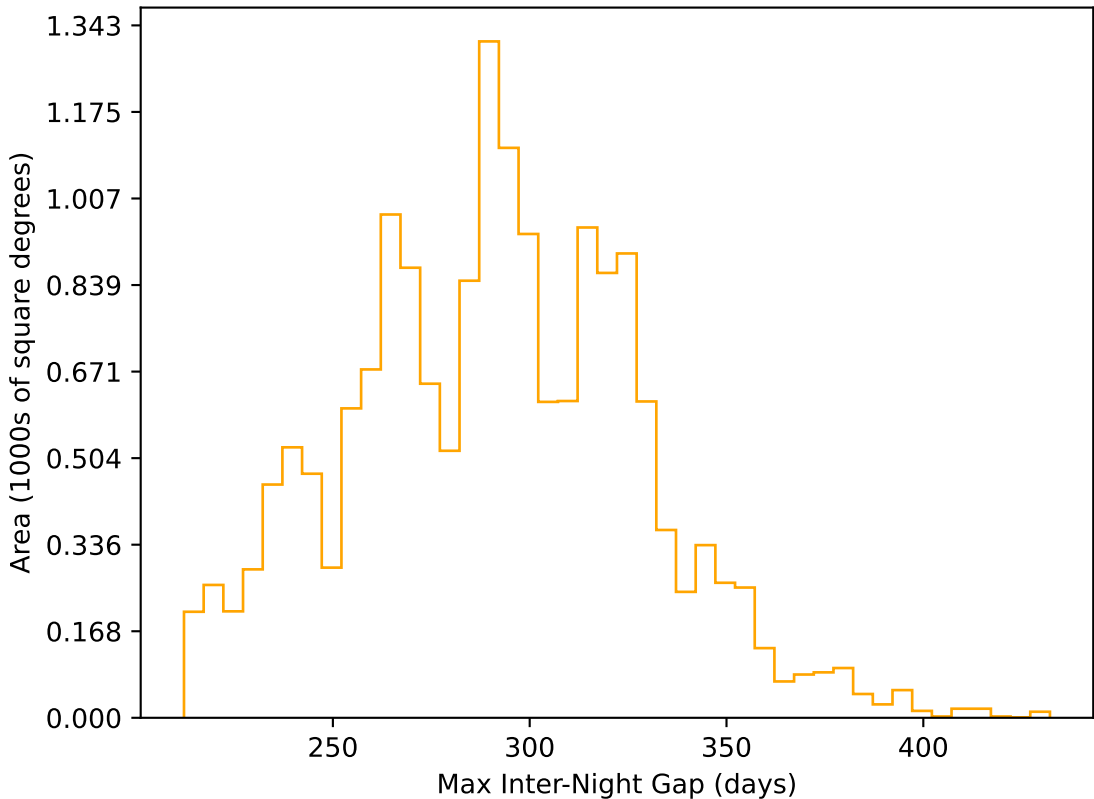
too_ignore_10_1v3.4_10yrs WFD r band: Max Inter-Night Gap
