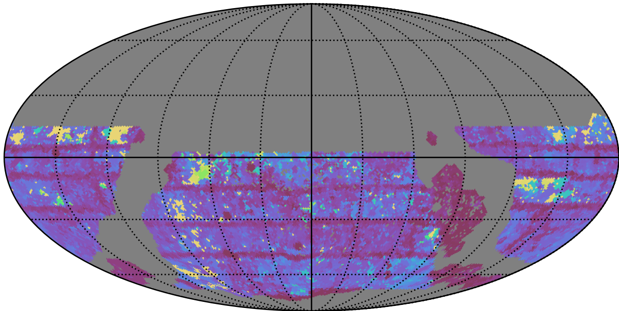
too_ignore_10_1v3.4_10yrs WFD i band: Max Inter-Night Gap
