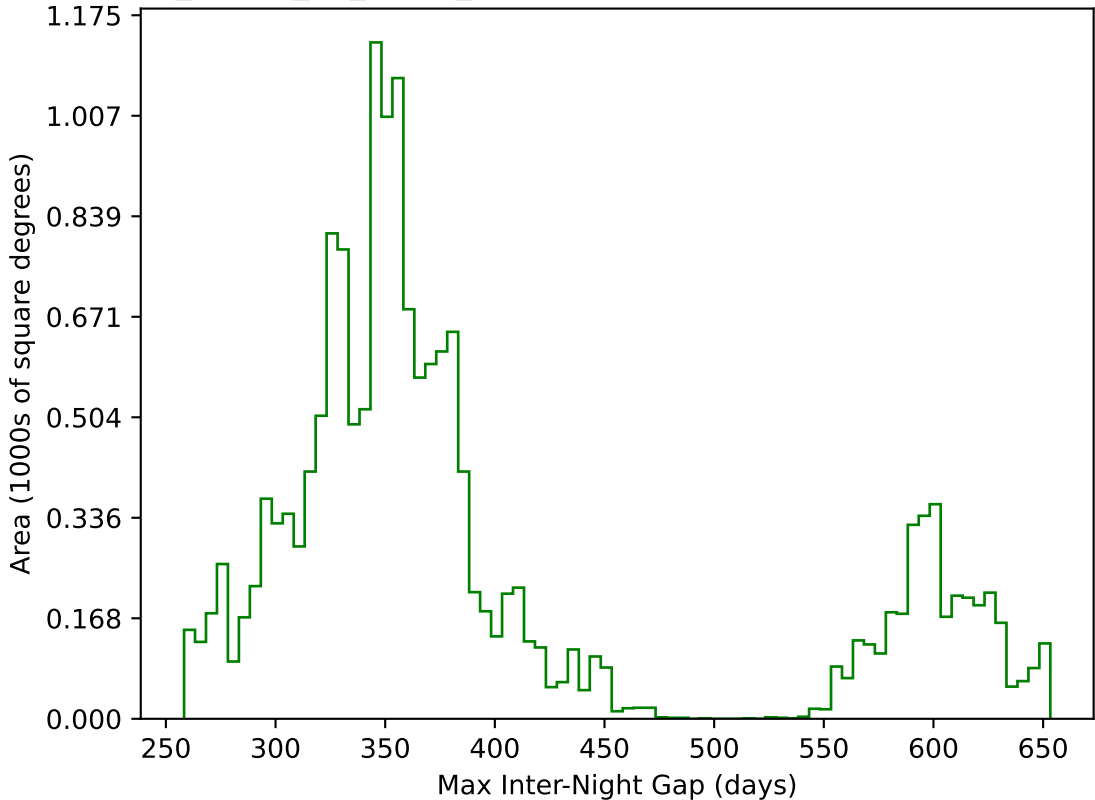
too_ignore_10_1v3.4_10yrs WFD g band: Max Inter-Night Gap
