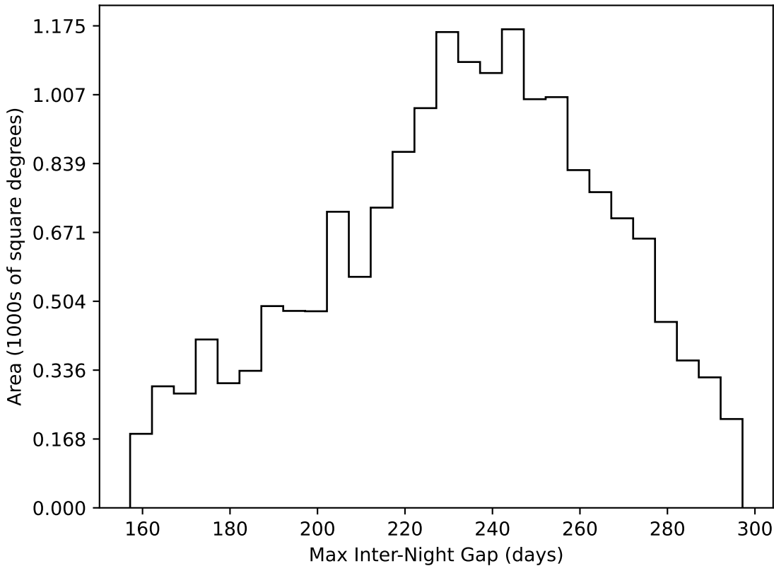
too_ignore_10_1v3.4_10yrs WFD all bands: Max Inter-Night Gap
