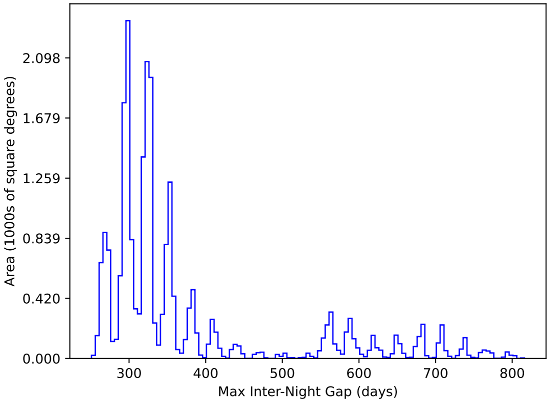
too_ignore_10_1v3.4_10yrs All sky y band: Max Inter-Night Gap
