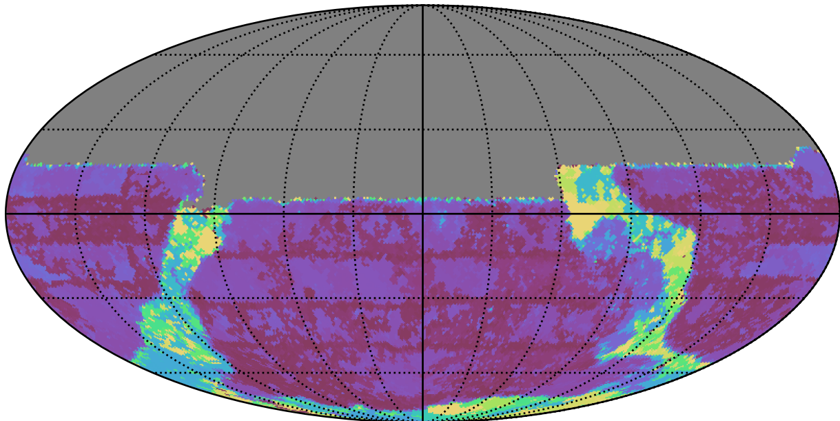
too_ignore_10_1v3.4_10yrs All sky u band: Max Inter-Night Gap
