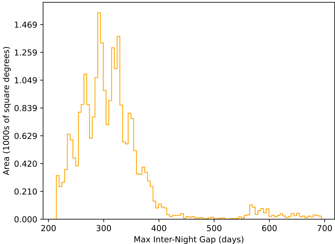
too_ignore_10_1v3.4_10yrs All sky r band: Max Inter-Night Gap
