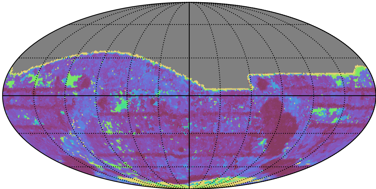
too_ignore_10_1v3.4_10yrs All sky i band: Max Inter-Night Gap
