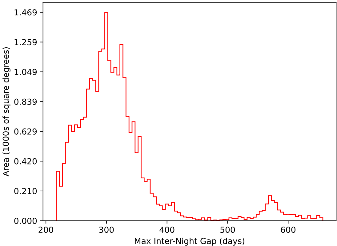
too_ignore_10_1v3.4_10yrs All sky i band: Max Inter-Night Gap
