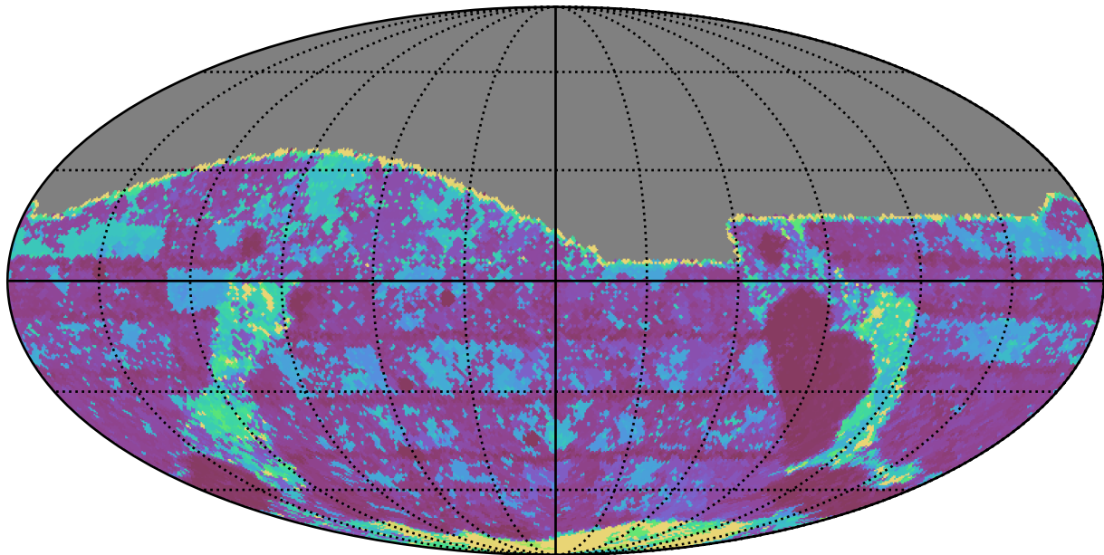
too_ignore_10_1v3.4_10yrs All sky g band: Max Inter-Night Gap
