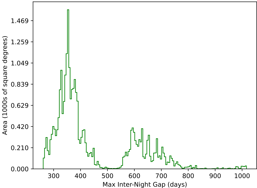
too_ignore_10_1v3.4_10yrs All sky g band: Max Inter-Night Gap
