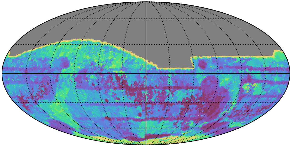
too_ignore_10_1v3.4_10yrs All sky all bands: Max Inter-Night Gap
