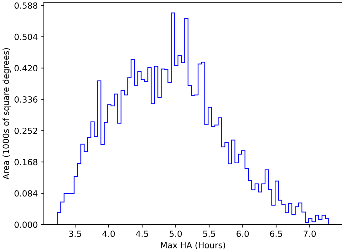
too_ignore_10_1v3.4_10yrs WFD z band: Max HA
