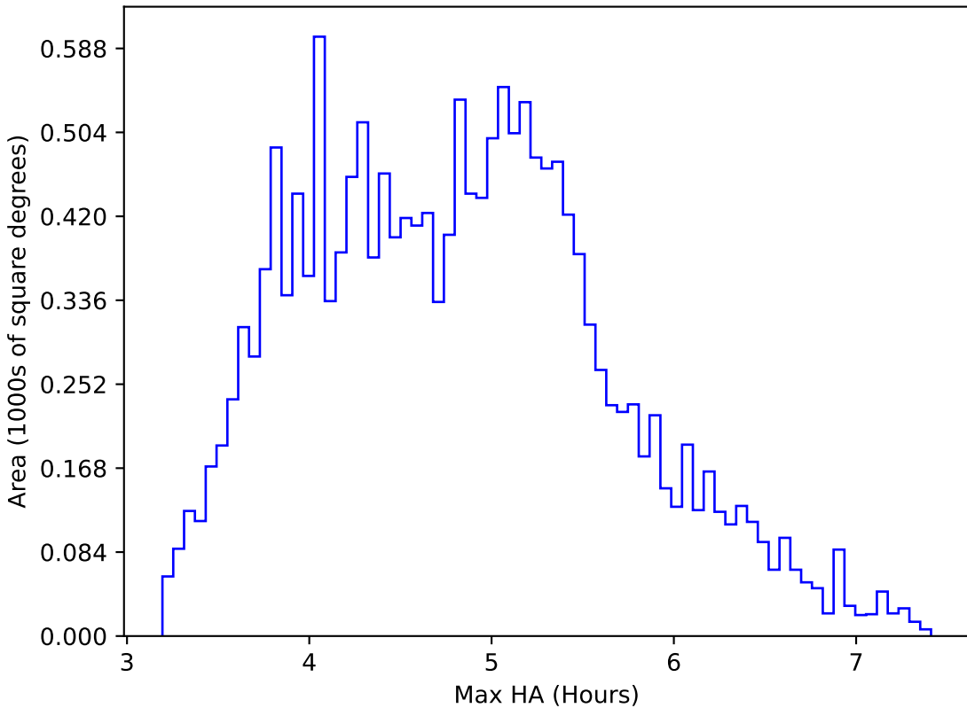
too_ignore_10_1v3.4_10yrs WFD i band: Max HA
