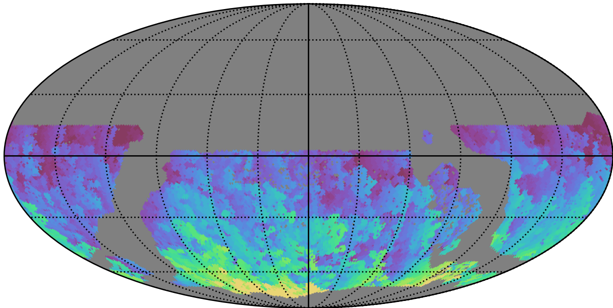
too_ignore_10_1v3.4_10yrs WFD g band: Max HA
