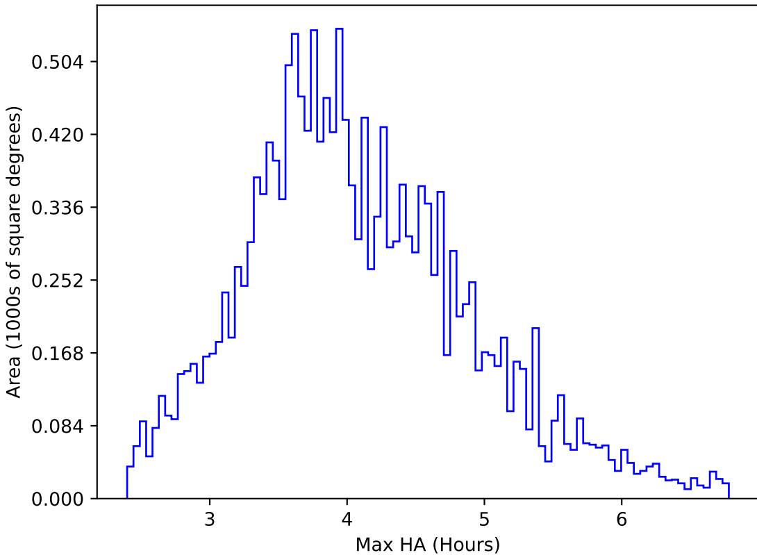
too_ignore_10_1v3.4_10yrs WFD g band: Max HA
