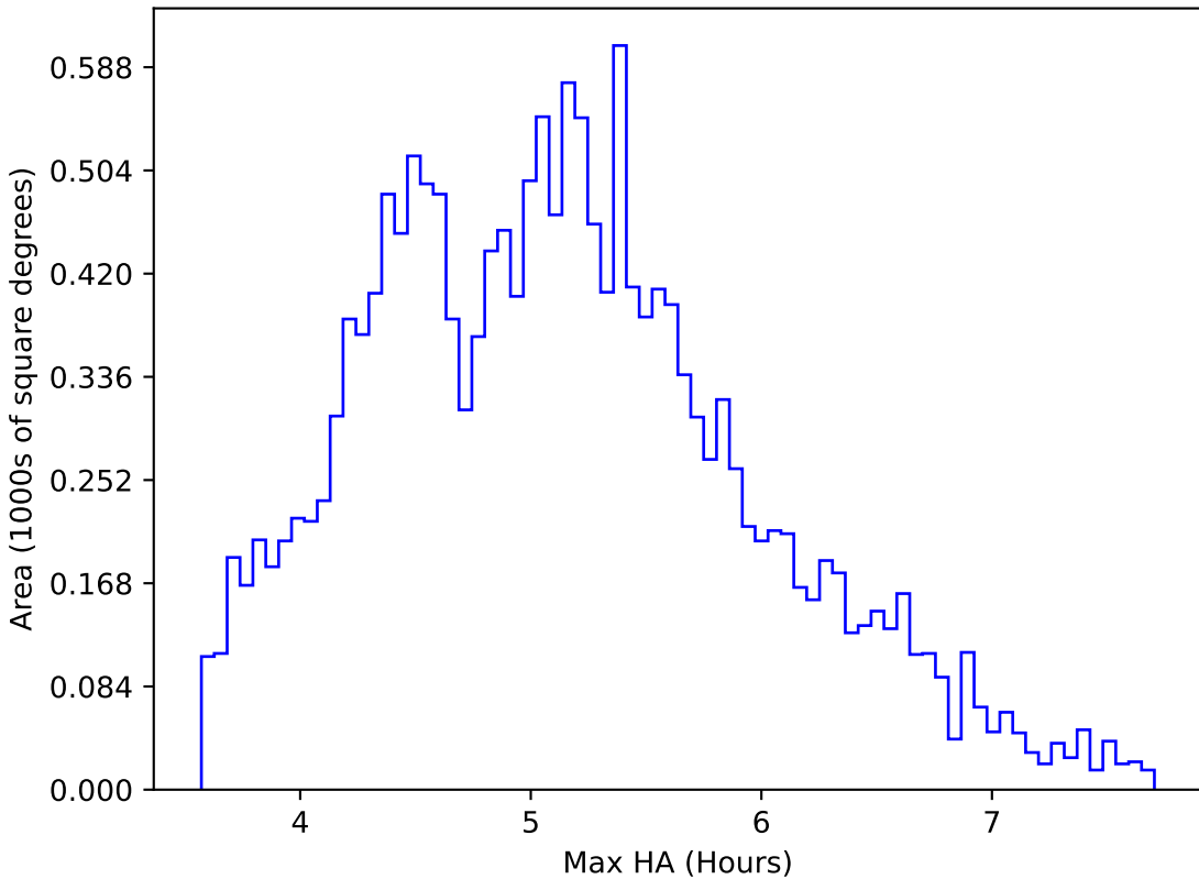
too_ignore_10_1v3.4_10yrs WFD all bands: Max HA
