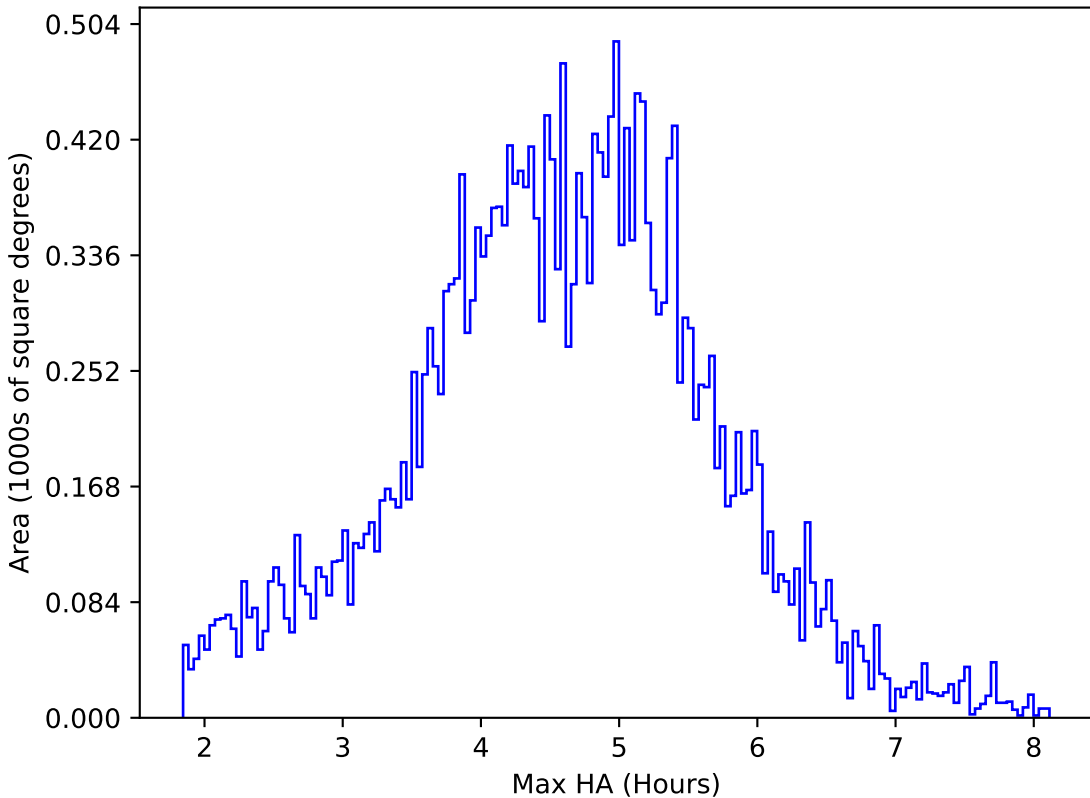
too_ignore_10_1v3.4_10yrs All sky z band: Max HA
