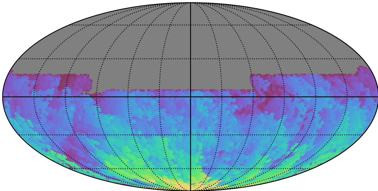
too_ignore_10_1v3.4_10yrs All sky u band: Max HA
