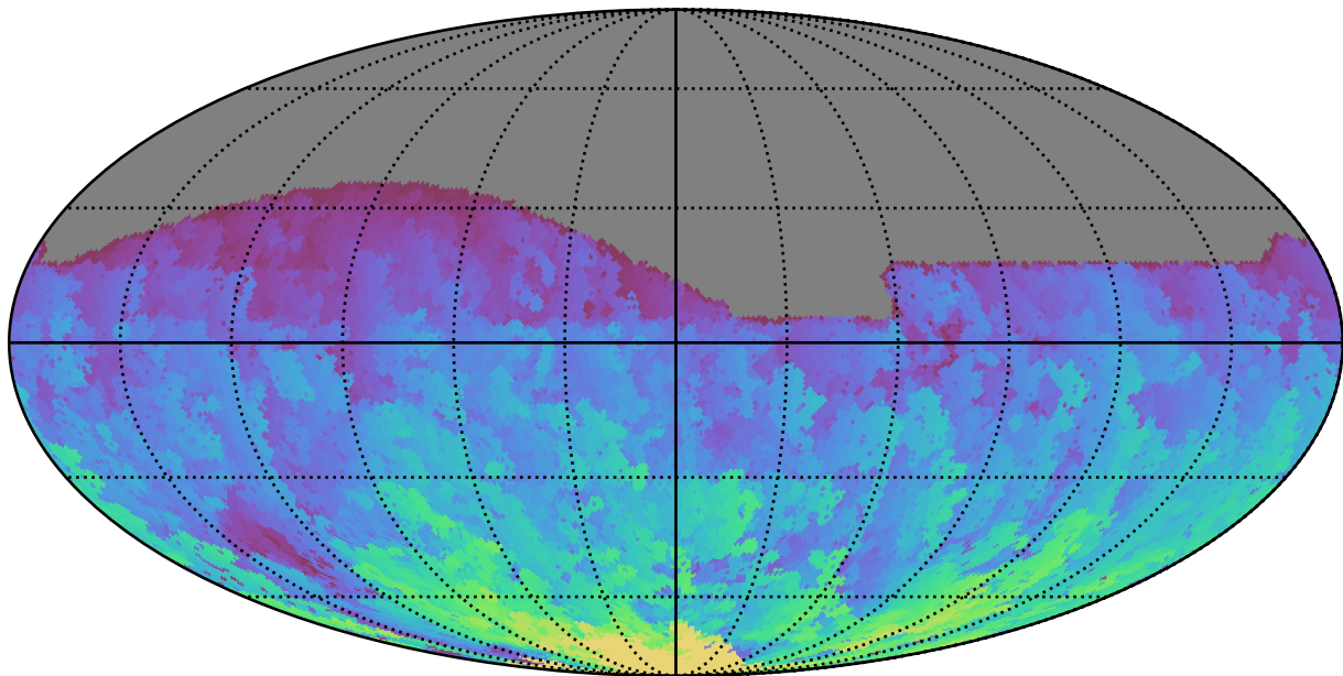
too_ignore_10_1v3.4_10yrs All sky g band: Max HA
