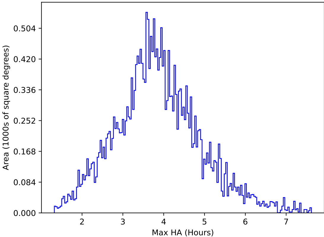
too_ignore_10_1v3.4_10yrs All sky g band: Max HA
