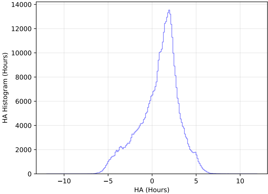
too_ignore_10_1v3.4_10yrs WFD z band: HA Histogram
